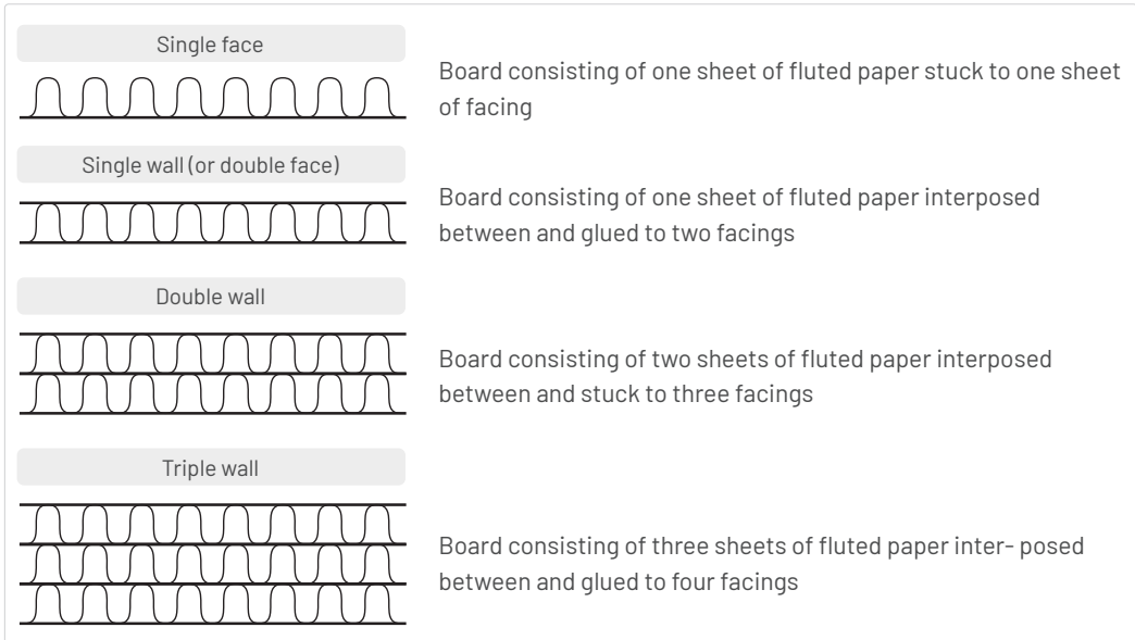
Figure 3: Corrugated board constructions
