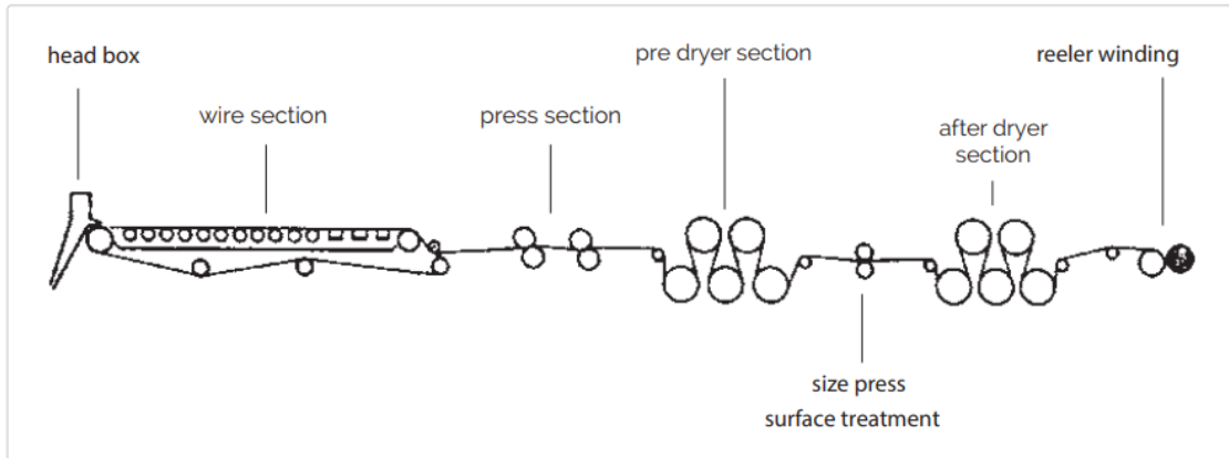
Figure 1: Example of paper machine for containerboard grades
